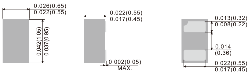
DFN 2L
