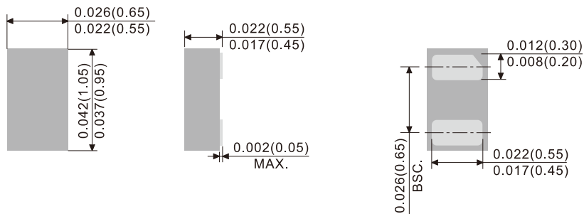
DFN1006-3L
