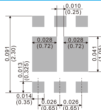
DFN2020-6L
