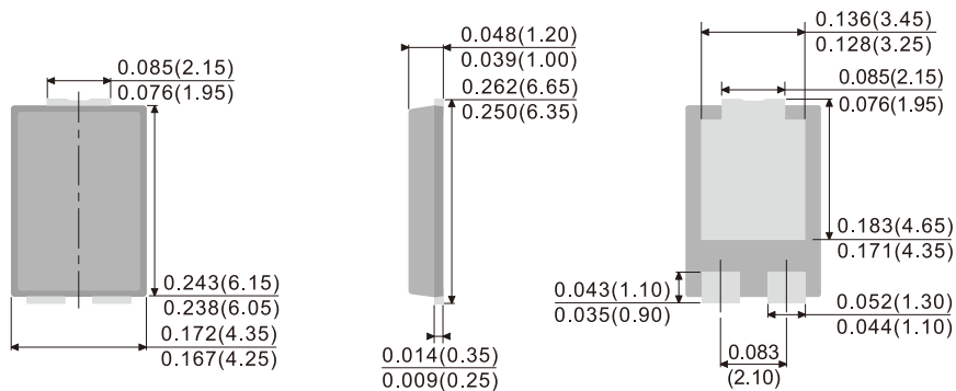
TO-277
