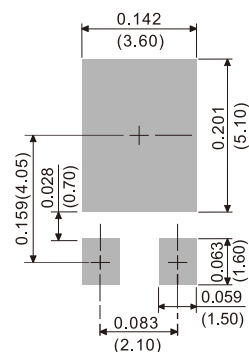
TO-277A
