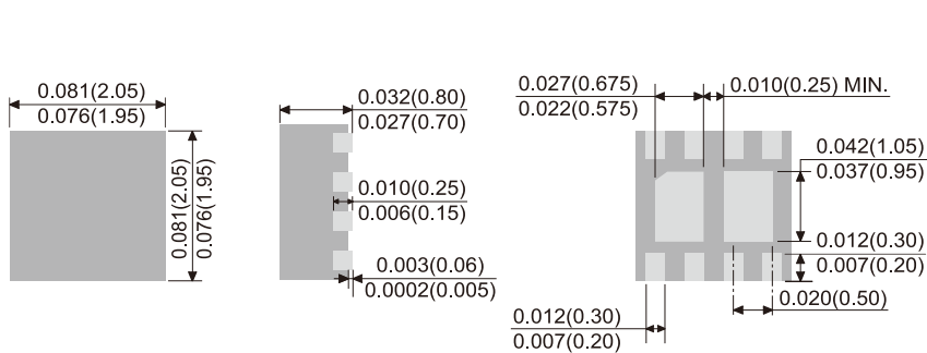
DFN2020-8L
