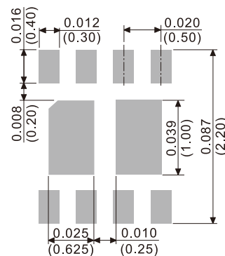
DFN2020-8L
