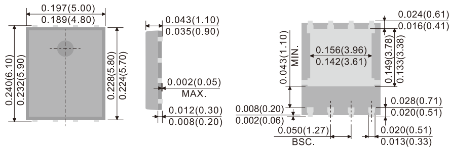
DFN5060B-8L
