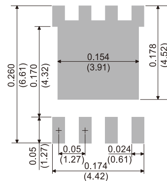
DFN5060B-8L
