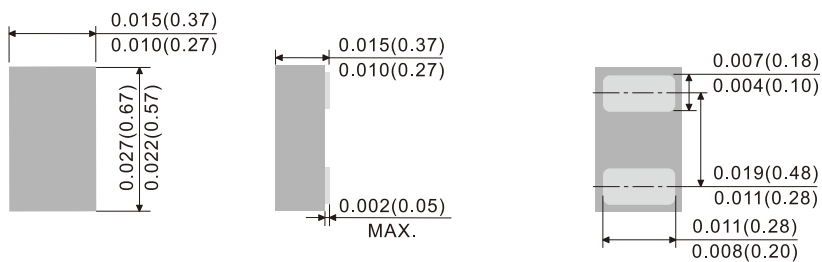
DFN0603-2L
