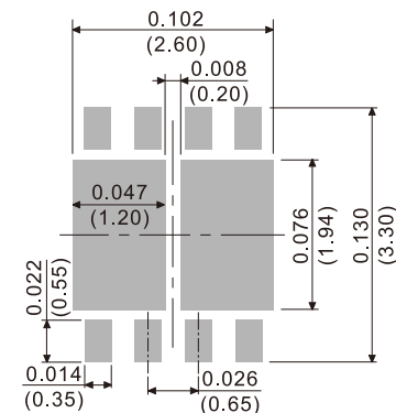
DFN3030B-8L
