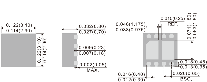
DFN3030B-8L
