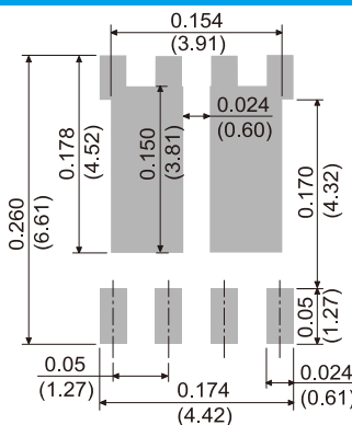
DFN5060B-8L
