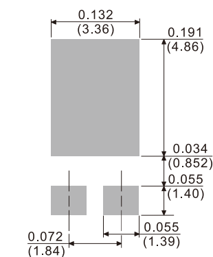
TO-277B
