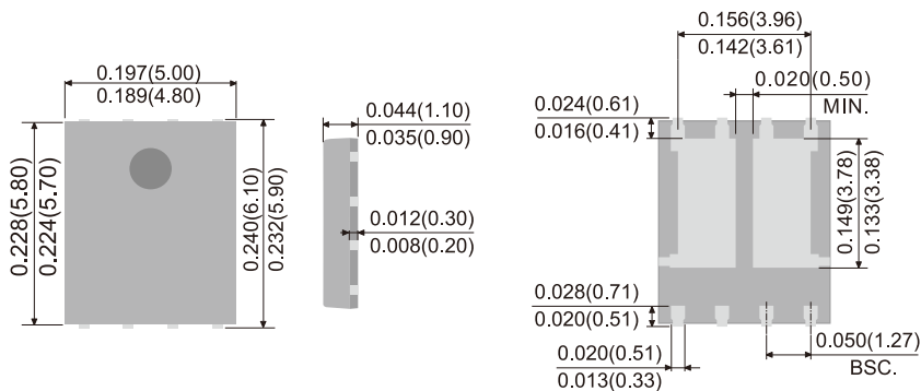
DFN5060B-8L
