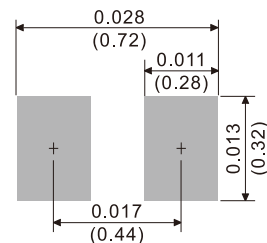
DFN0603
