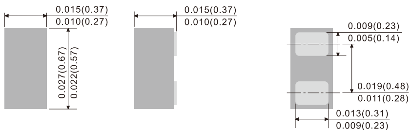
DFN0603
