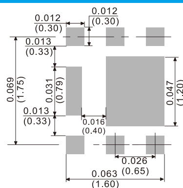
DFN2020B-6L
