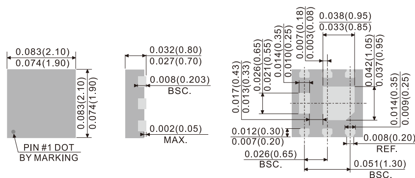
DFN2020B-6L
